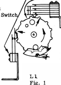
Replay Cams shown in their normal Indexed Positions. Switches are Open. Arrows point to Lobes that will actuate Switches.
