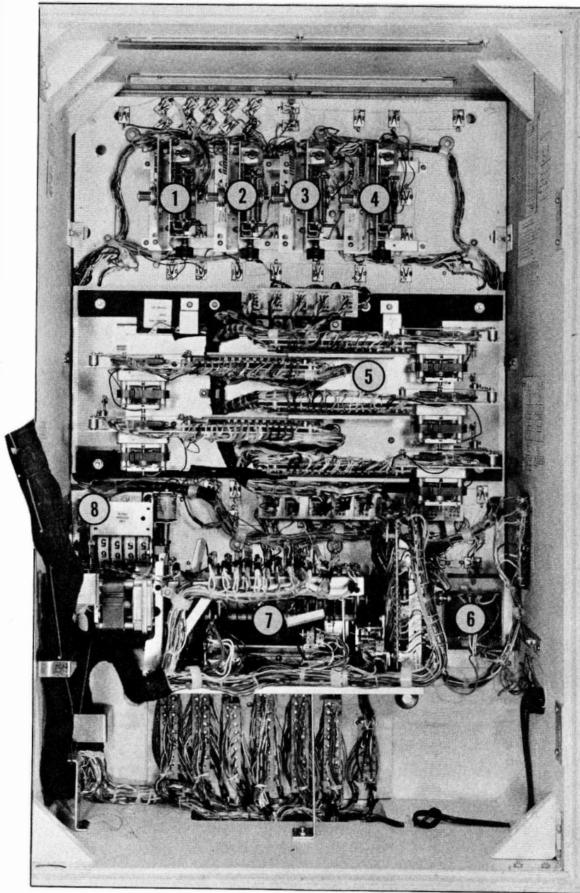
INSERT ASSEMBLY
